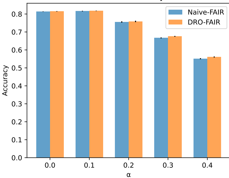
CREDIT - Accuracy
