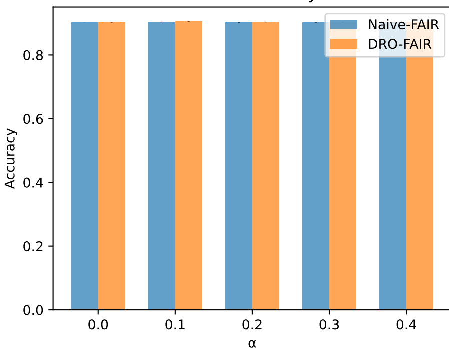
LSAC - Accuracy
