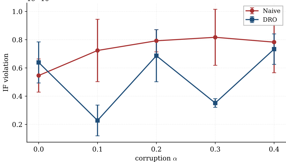
Adult IF violation vs \alpha — COMBINED attack ( \tau=1 )
