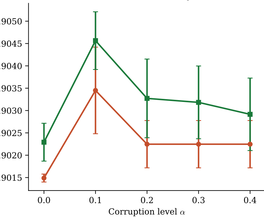
LSAC — Accuracy
