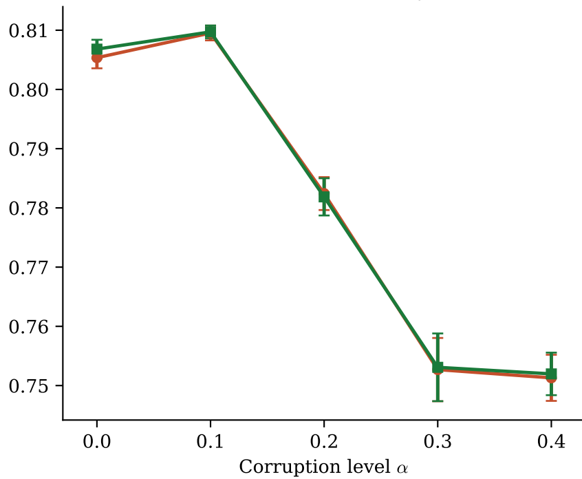
Credit — Accuracy
