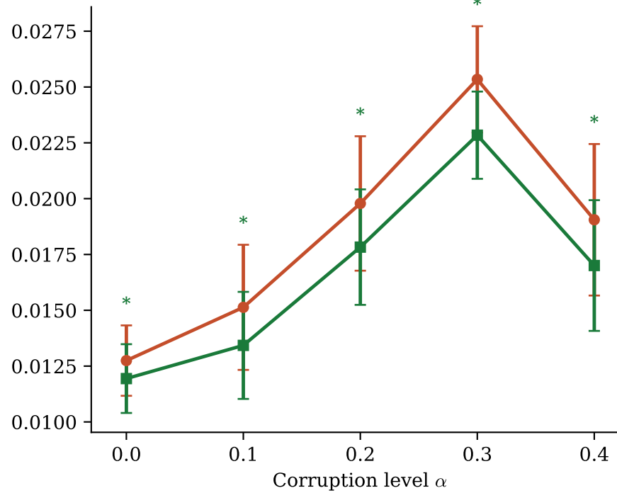
Credit — DP Violation ( \Delta_{DP} )
