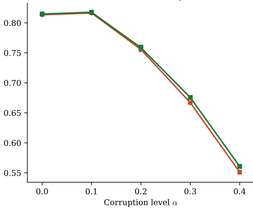
Adult — Accuracy
