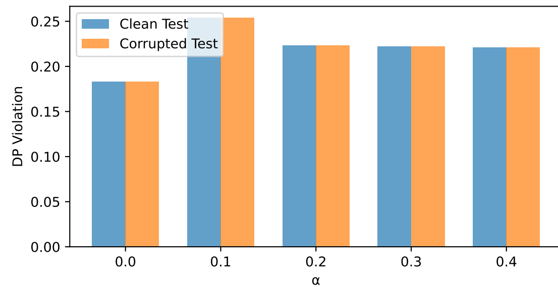
LSAC - DRO
