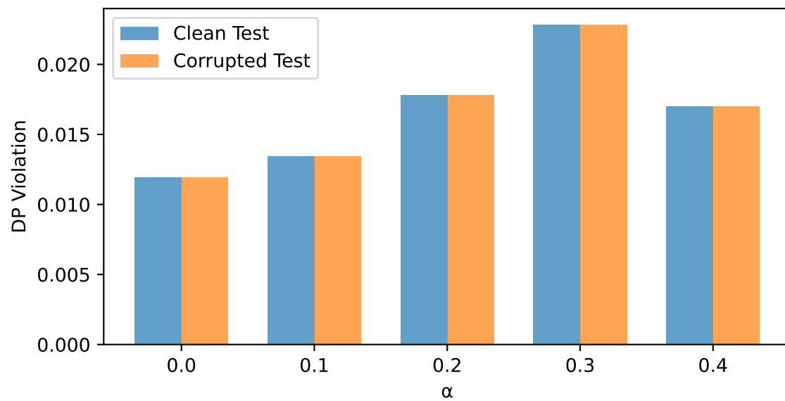
LSAC - DRO
