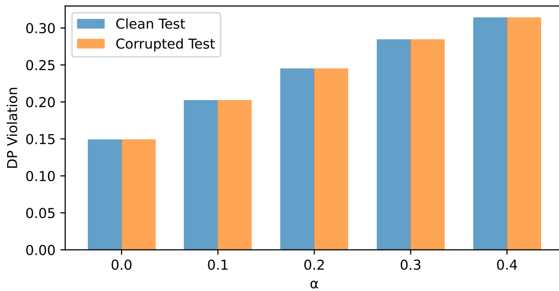
CREDIT - NAIVE
