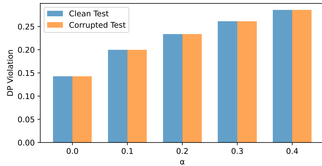
CREDIT - DRO
