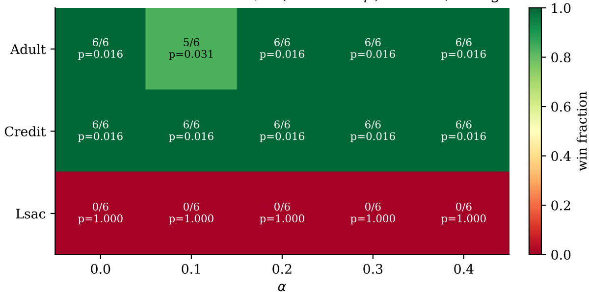
DP attack: DRO win count / 6 (Wilcoxon p ) — \tau = 1 , 540-grid
