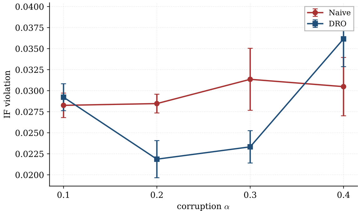
Adult IF violation vs \alpha ( \tau=100 )
