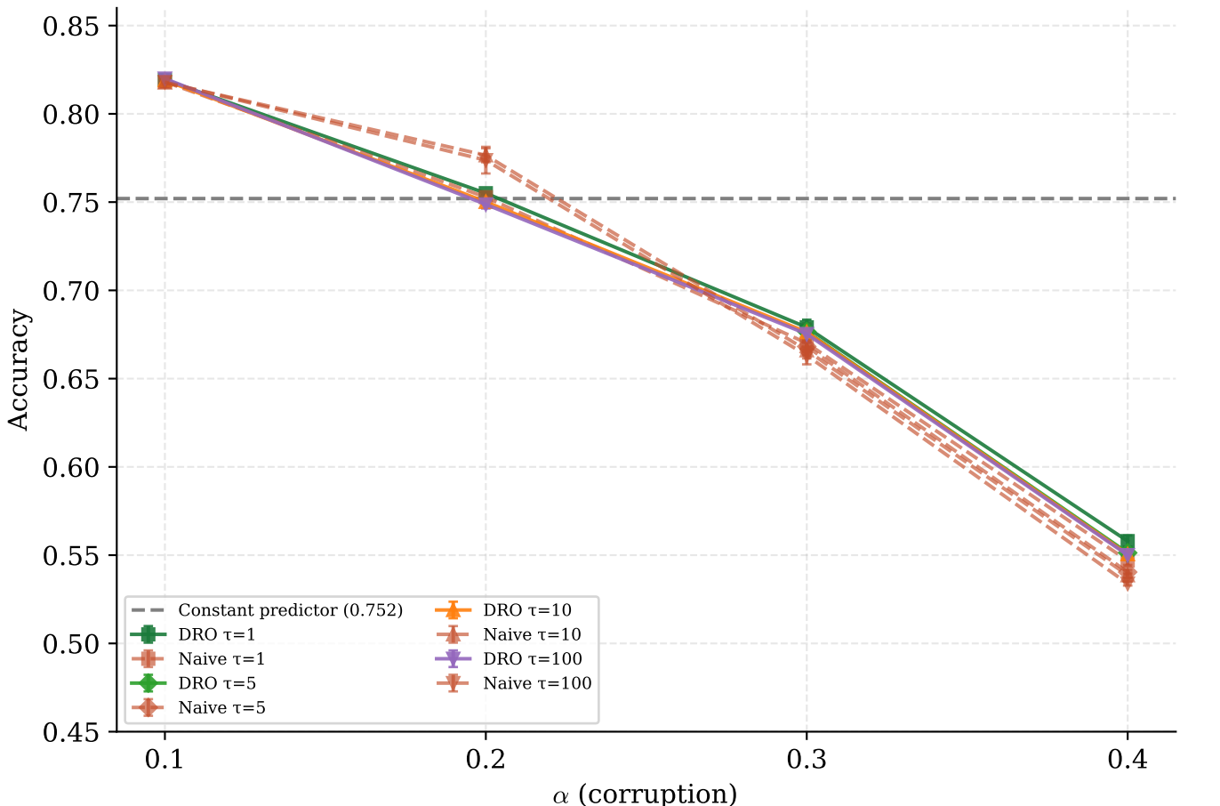
Constant predictor accuracy (Adult DP attack pref.) x=\alpha , lines diff \tau + Naive + 0.752 line
