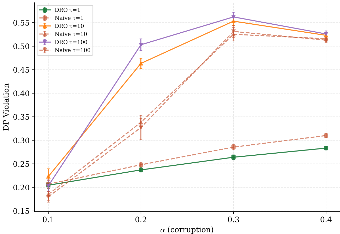
Constant predictor DP (Adult DP attack) x=\alpha lines for \tau + Naive
