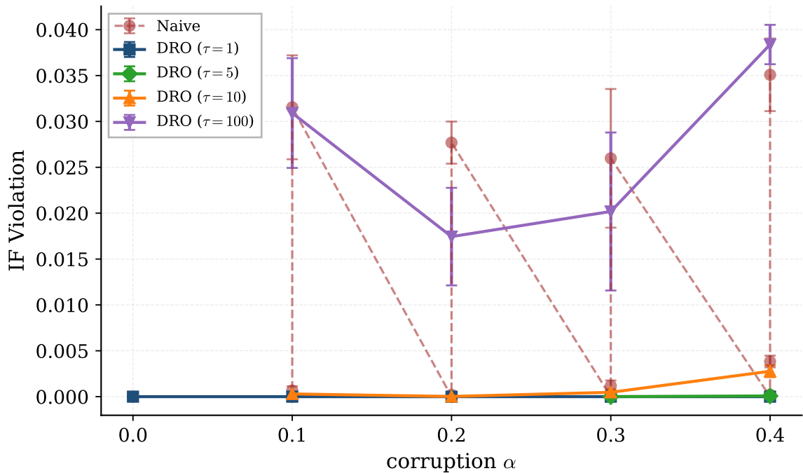
IF Violation vs \alpha — Adult (attack=DP)
