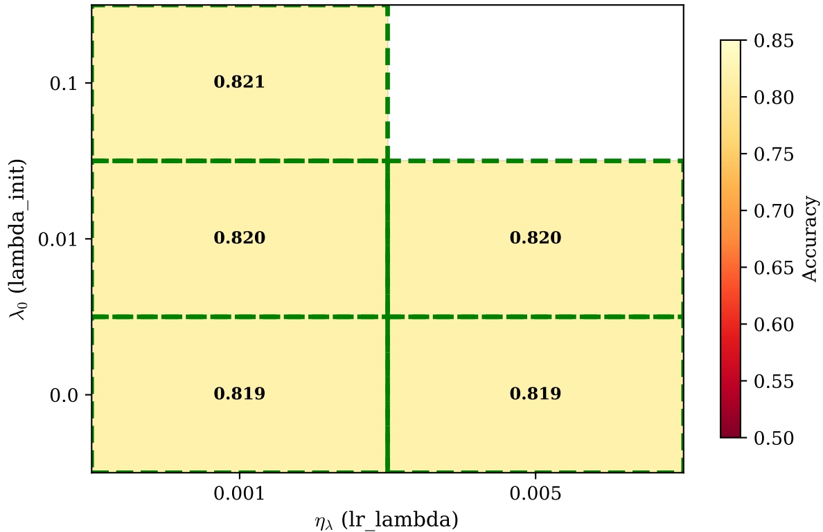
Accuracy — \lambda grid (Adult, \alpha=0.1 , attack=DP)
