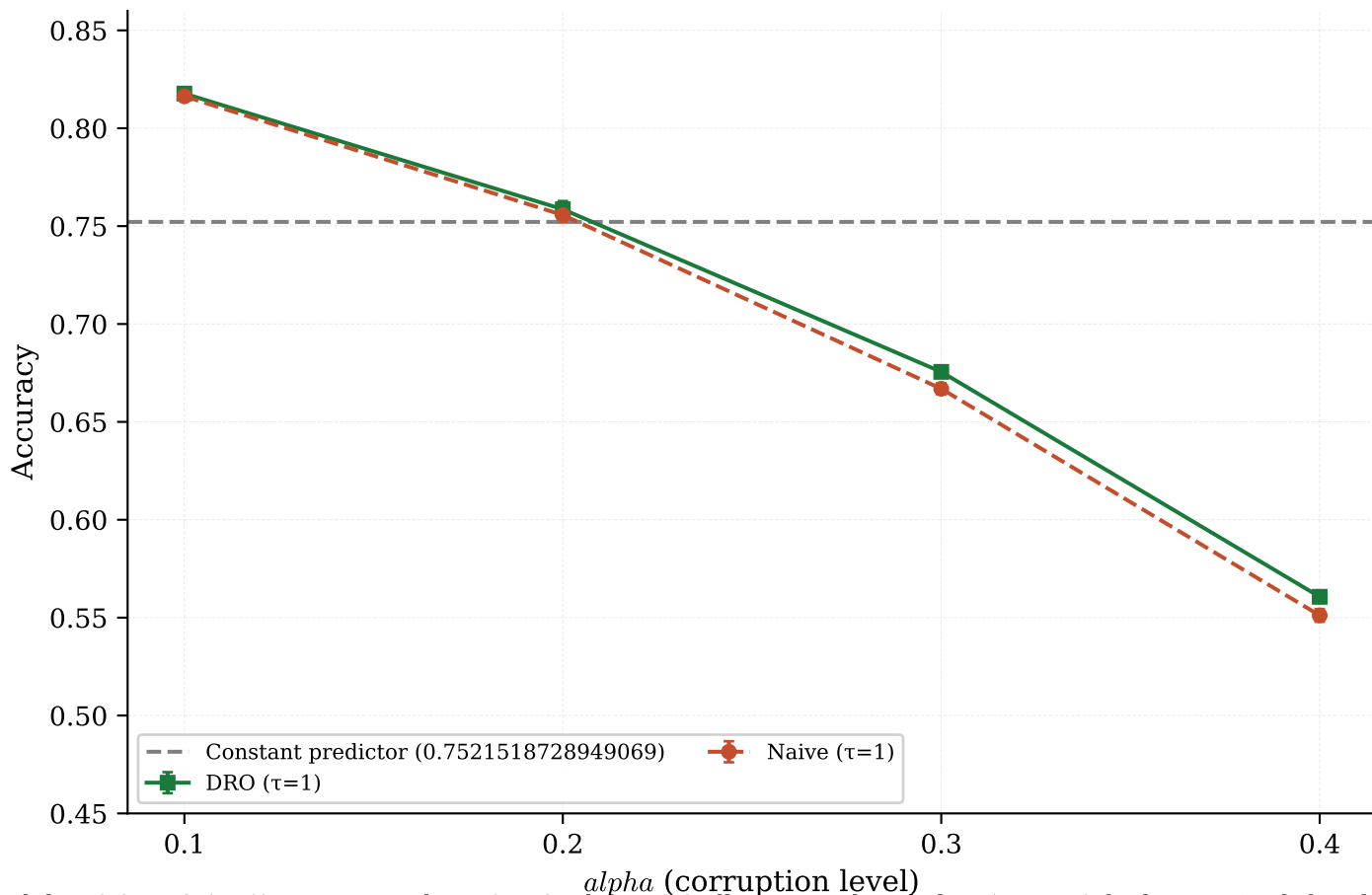
Constant-predictor accuracy figure (Adult, DP attack) x=\alpha ; lines for \tau + Naive + horiz 0.752
