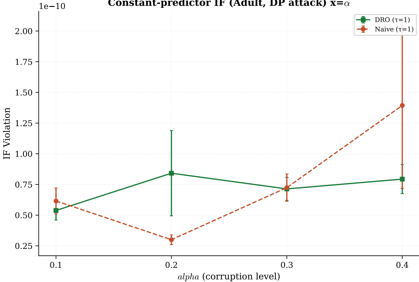
Constant-predictor IF (Adult, DP attack) x=\alpha
