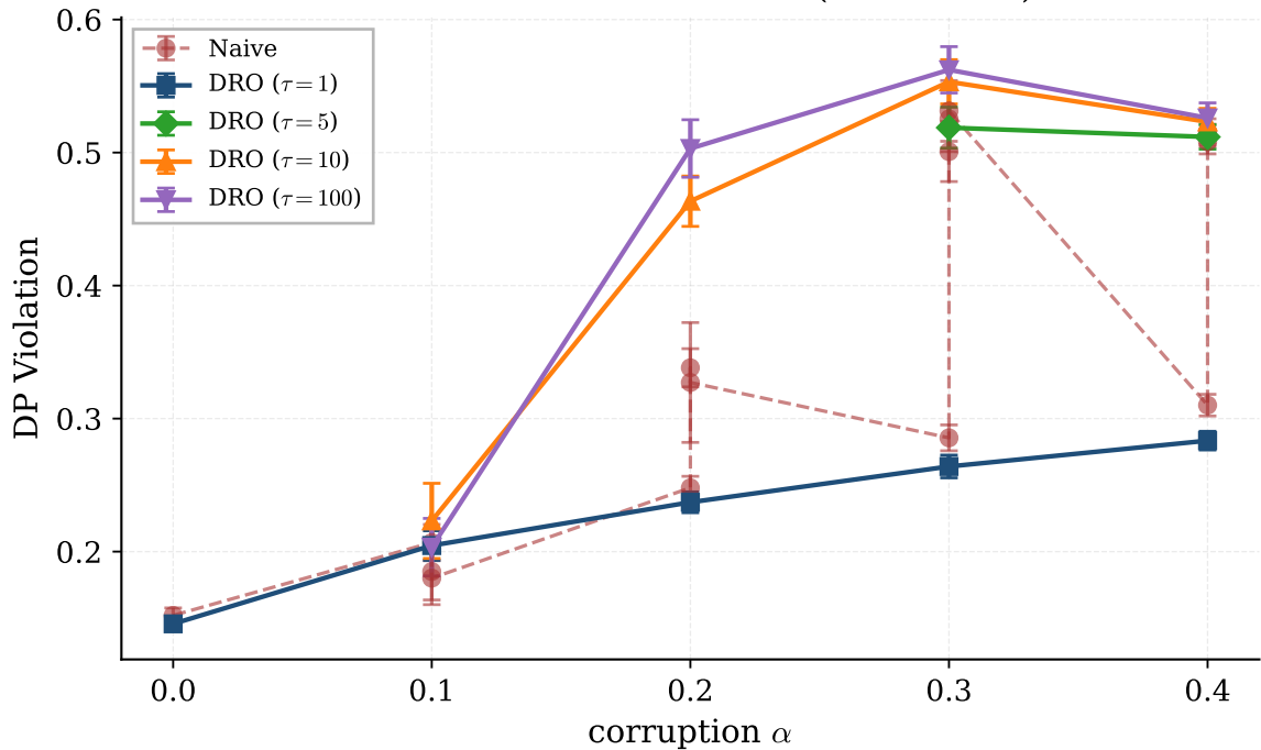
DP Violation vs \alpha — Adult (attack=DP)
