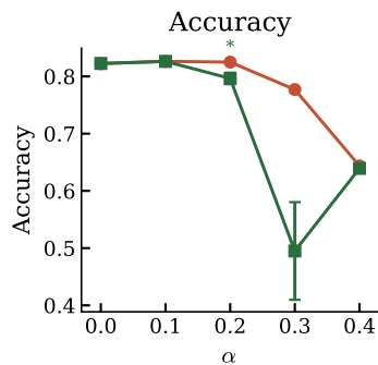
Adult
