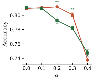
Credit
