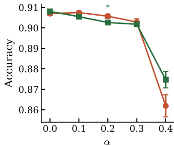
LSAC
