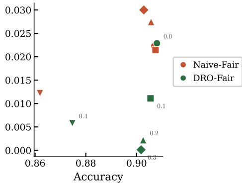
LSAC
