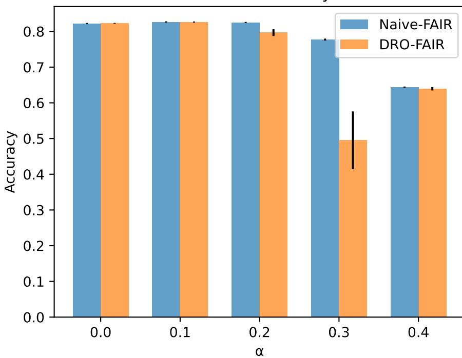
CREDIT - Accuracy
