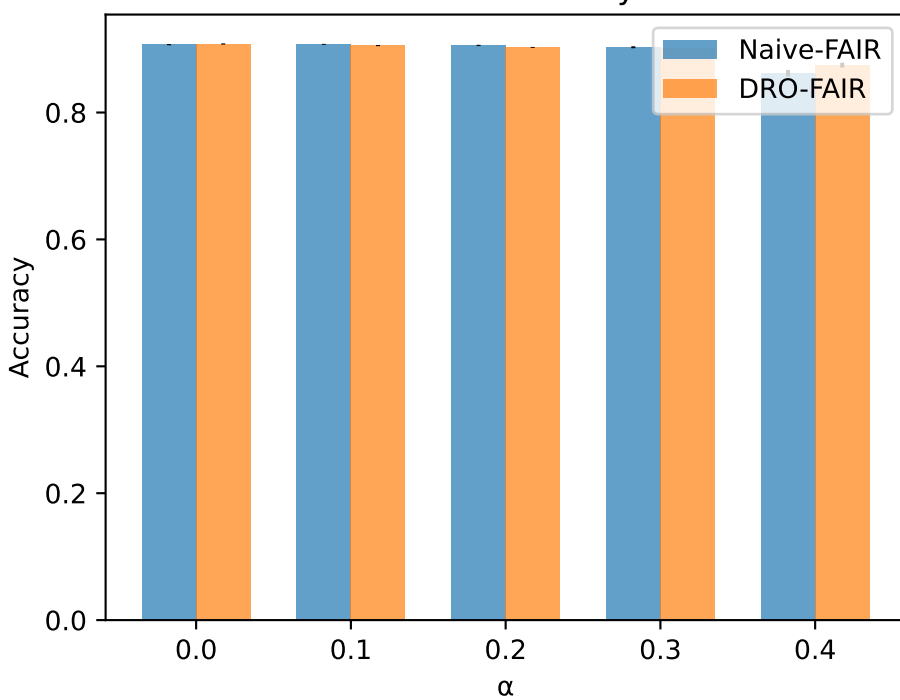
LSAC - Accuracy
