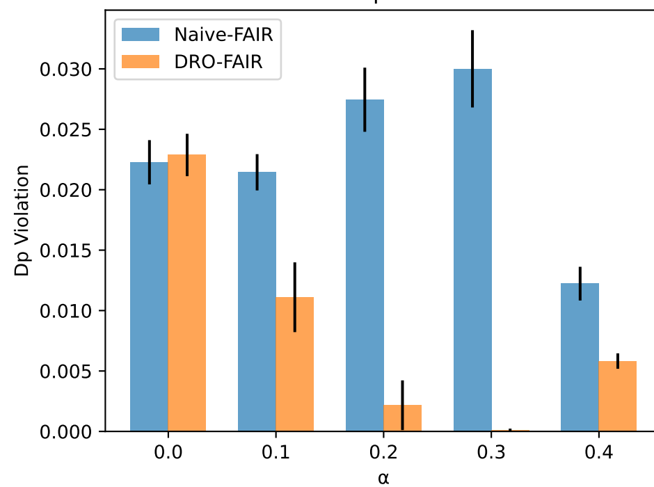
LSAC - Dp Violation
