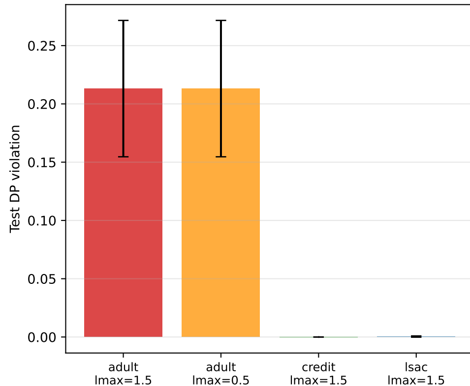
Final test DP (lower = fairer)
