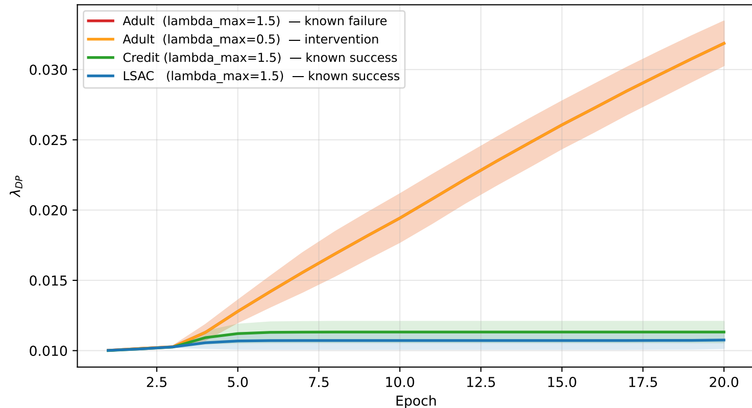
\lambda_{DP} trajectory (alpha=0.2, DP attack, 3 seeds)
