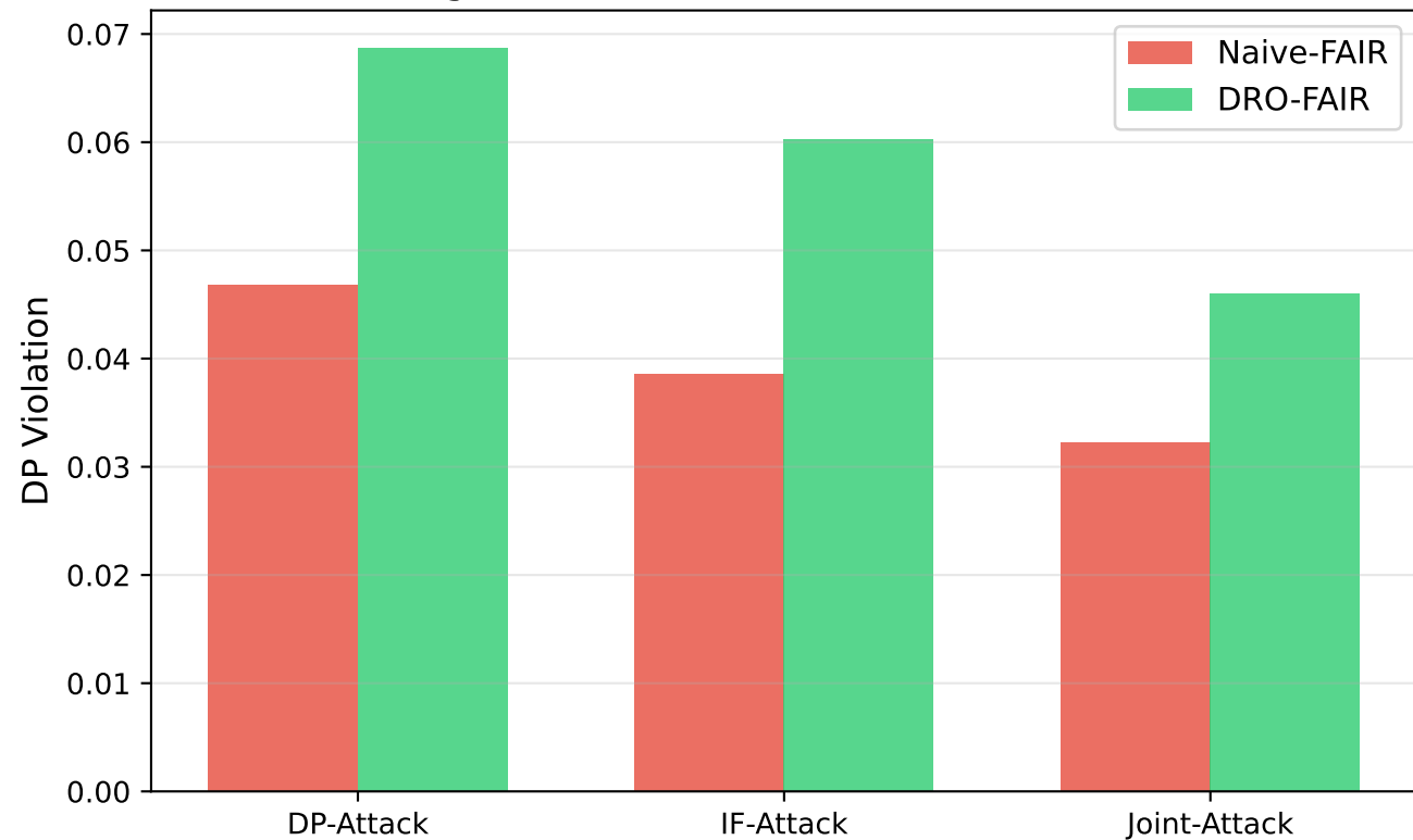
Fairness-Targeted PGD Attack on Adult ( \alpha=0.2 , Smoke Test)
