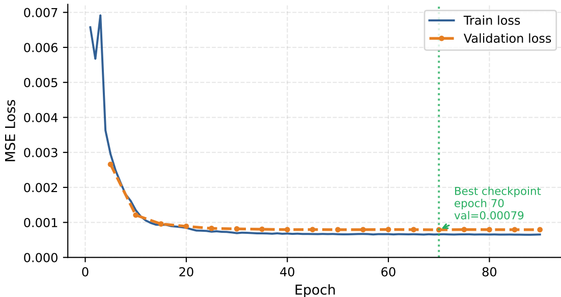
CASCADE EvolveGCN-H — Training Convergence
