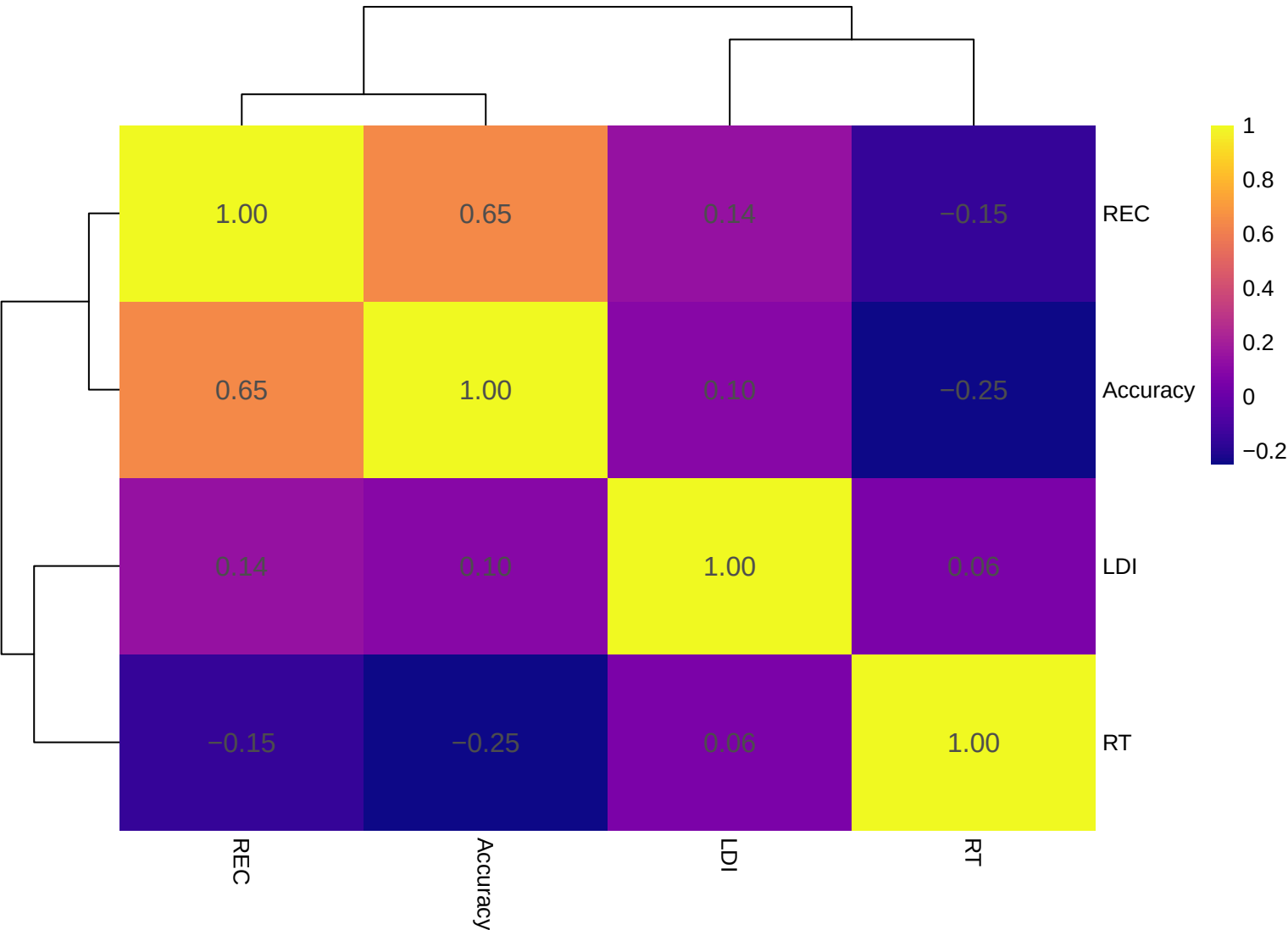
Core Metric Correlations
