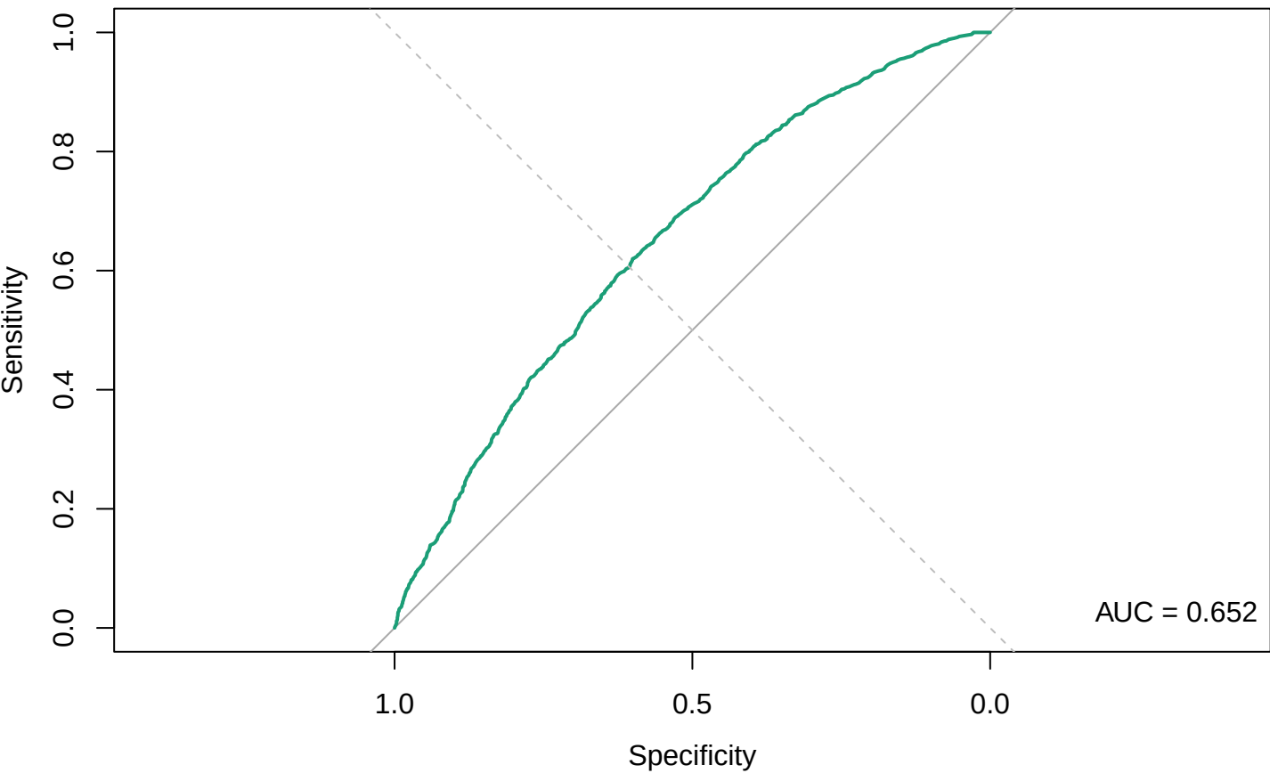
GLMM Target ROC Curve
