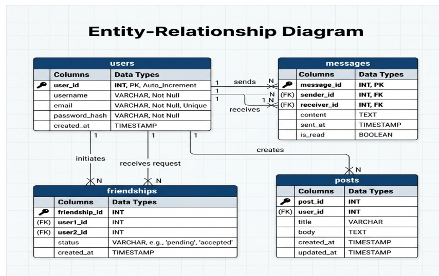
Figure 3.2: Database Entity-Relationship Diagram.
