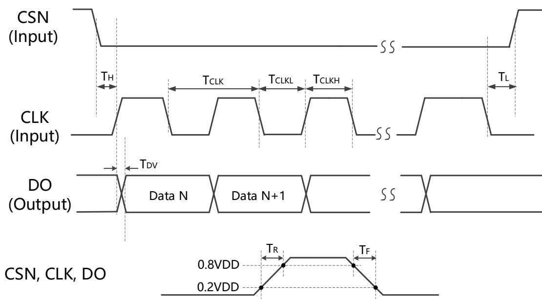
Figure-24: SSI Timing Diagram
