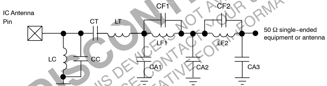
Figure 12. Structure of the Single-ended Antenna Interface for TX Operation to 50 \Omega Single-ended Equipment or Antenna
