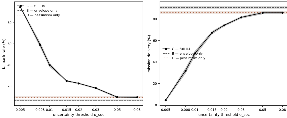
Figure 3. Campaign P2.3 (300 runs per point). Left: fallback rate of arm C against the uncertainty threshold (95 % CI), with arms B and D as horizontal references. Right: mission delivery on the same grid. The D reference isolates the cost of pessimistic evaluation; the vertical distance from D to the C curve is the cost of the uncertainty threshold itself.
