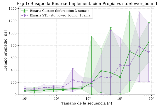
(b) Binaria Custom vs std::lower_bound .
