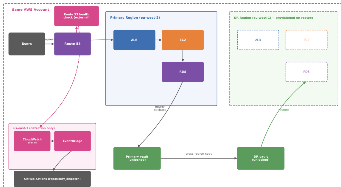
Figure 3. Full network architecture — primary/DR regions and the detection path isolated in a third region.
