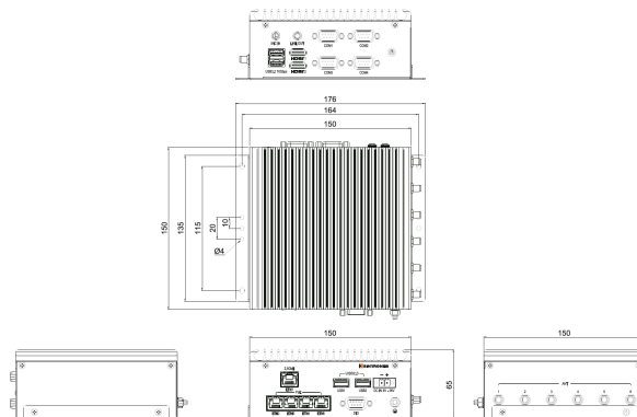
SBOX-2624P
