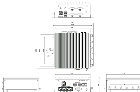
SBOX-2624P
