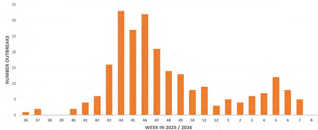
Number of outbreaks per week 01/09/2025 to 17/02/2026
