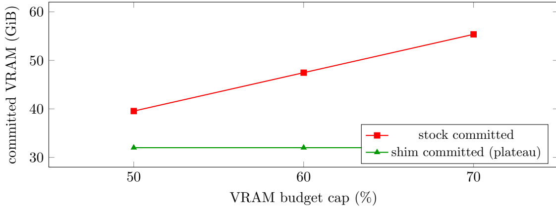
Figure 3: Committed bytes vs budget. Shim hits slot/commit plateau before consuming the full 70% budget cap.
