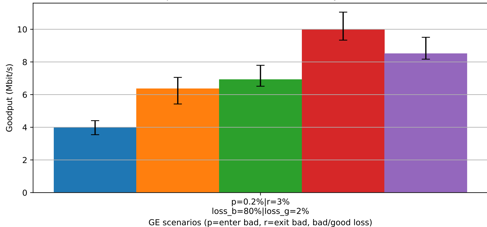
Goodput under GE — Data=50MB, delay1=10ms
