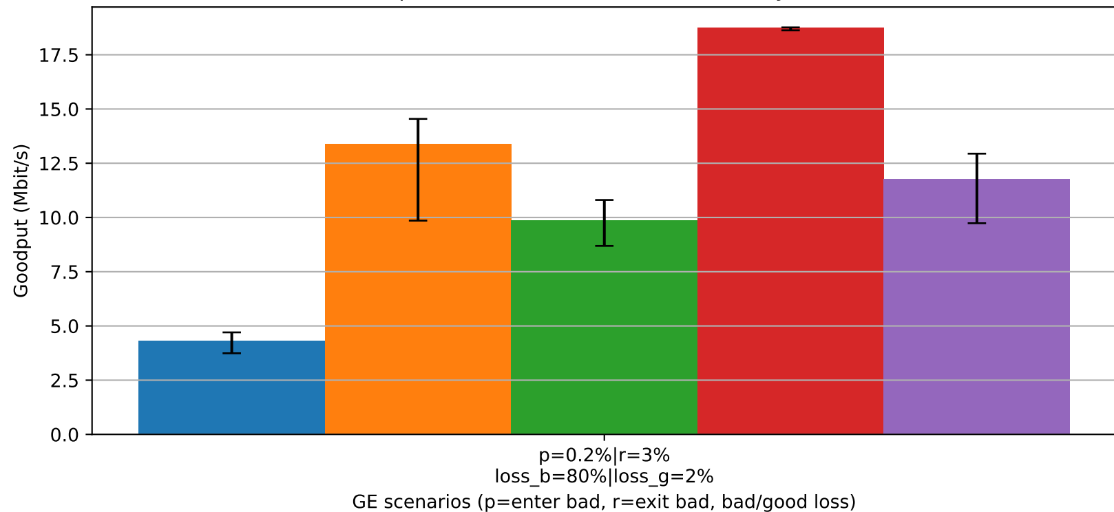
Goodput under GE — Data=50MB, delay1=2ms
