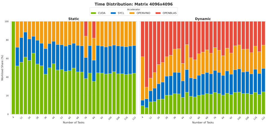
Figure 5.12: Time Distribution 4096
