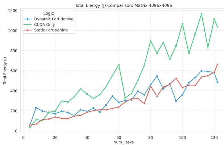
Figure 5.10: Energy Comparison 4096
