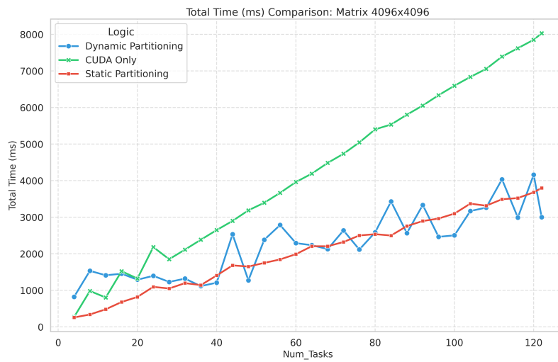
Figure 5.9: Time Comparison 4096
