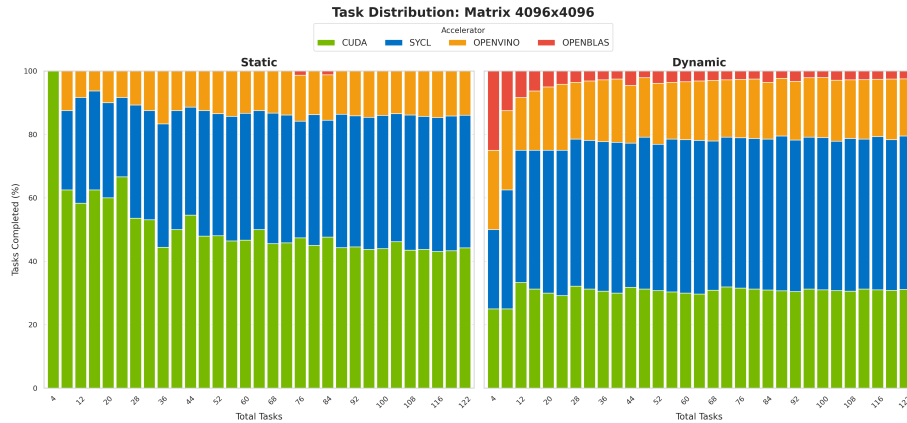
Figure 5.11: Task Distribution 4096
