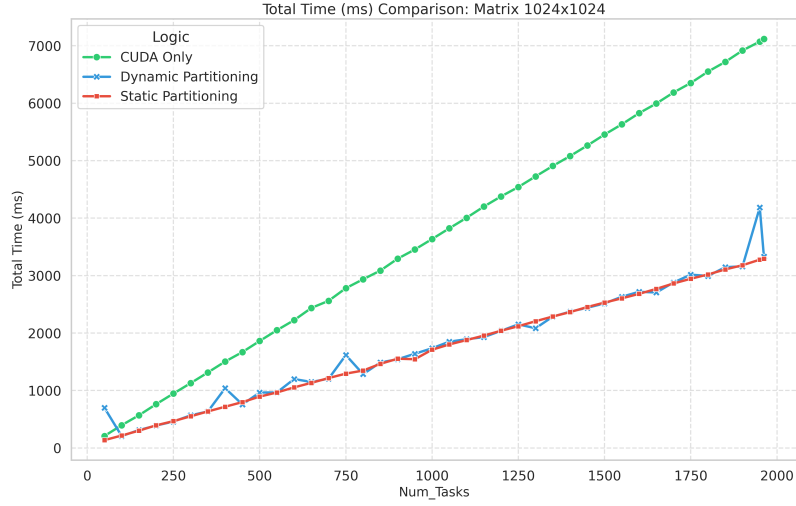
Figure 5.1: Time Comparison 1024
