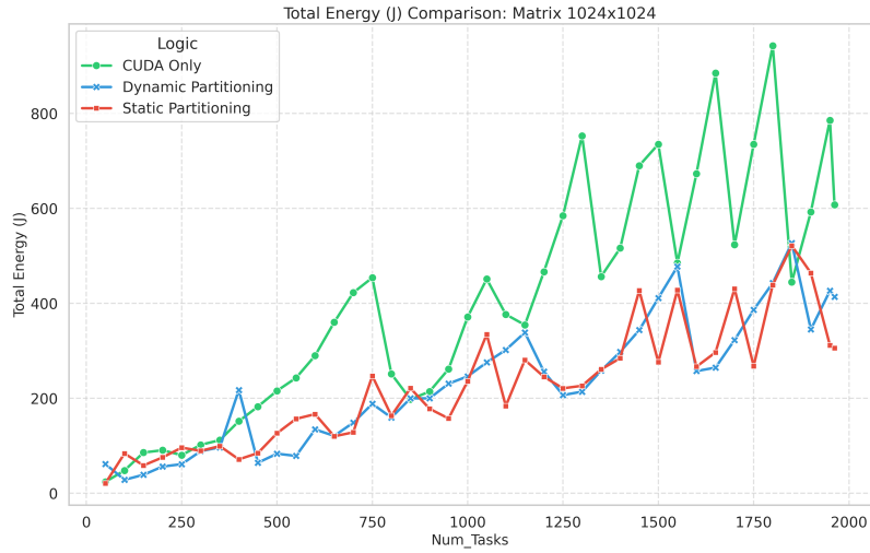
Figure 5.2: Energy Comparison 1024
