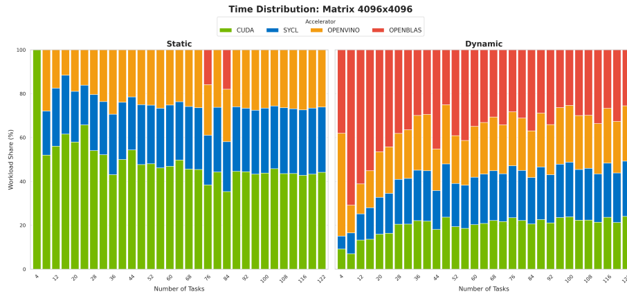
Figure 5.12: Time Distribution 4096
