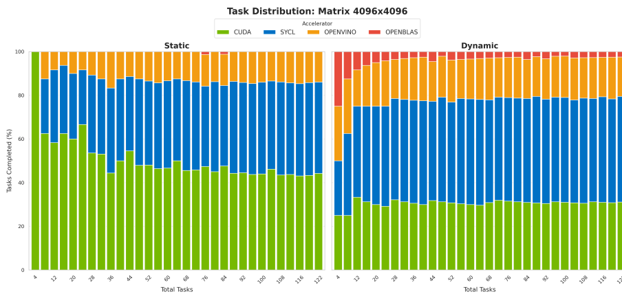
Figure 5.11: Task Distribution 4096
