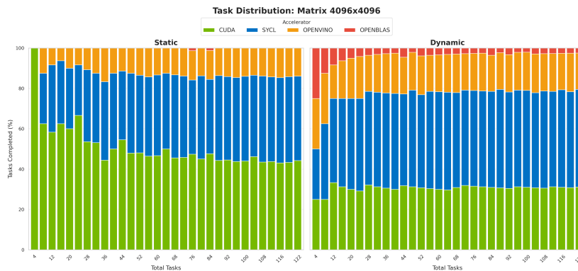
Figure 5.11: Task Distribution 4096
