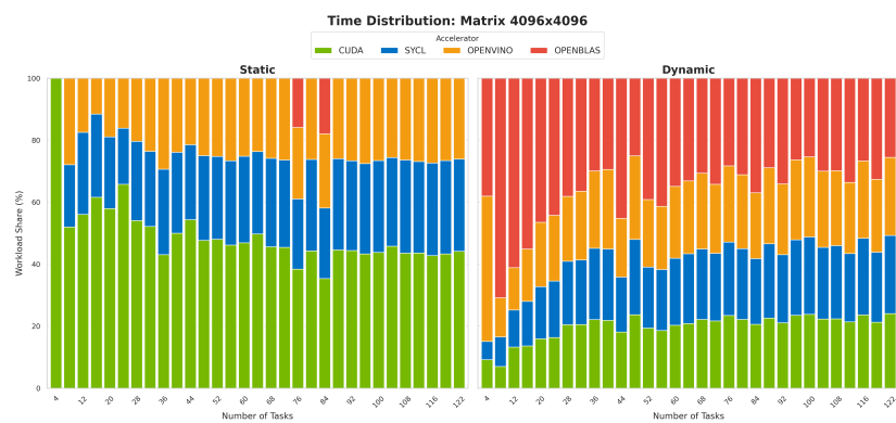
Figure 5.12: Time Distribution 4096
