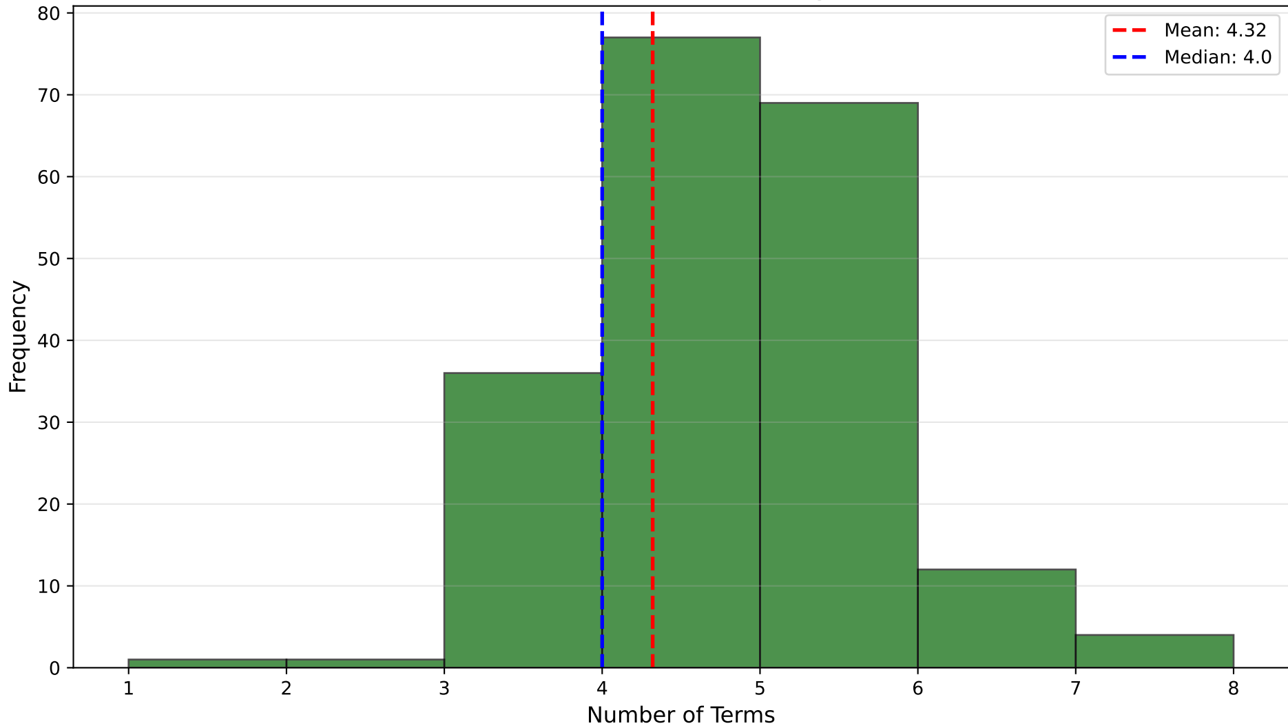
4-Variable K-Maps (70% Density, 16 cells)
