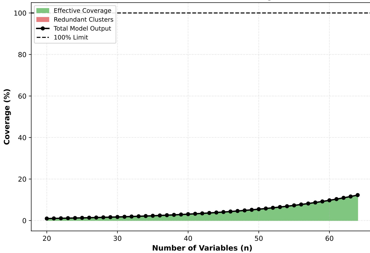
Cluster Growth
