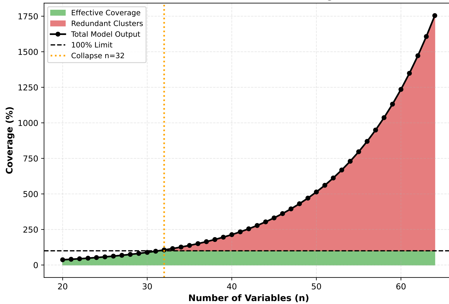
Cluster Growth
