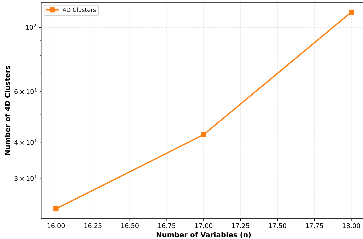
Cluster Growth
