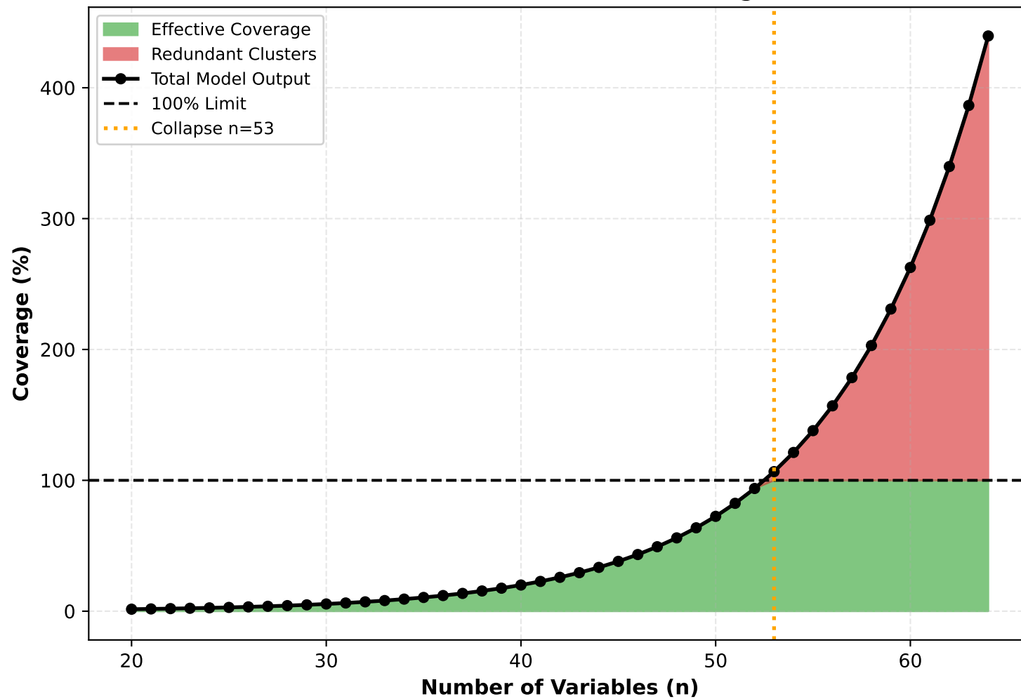
Cluster Growth
