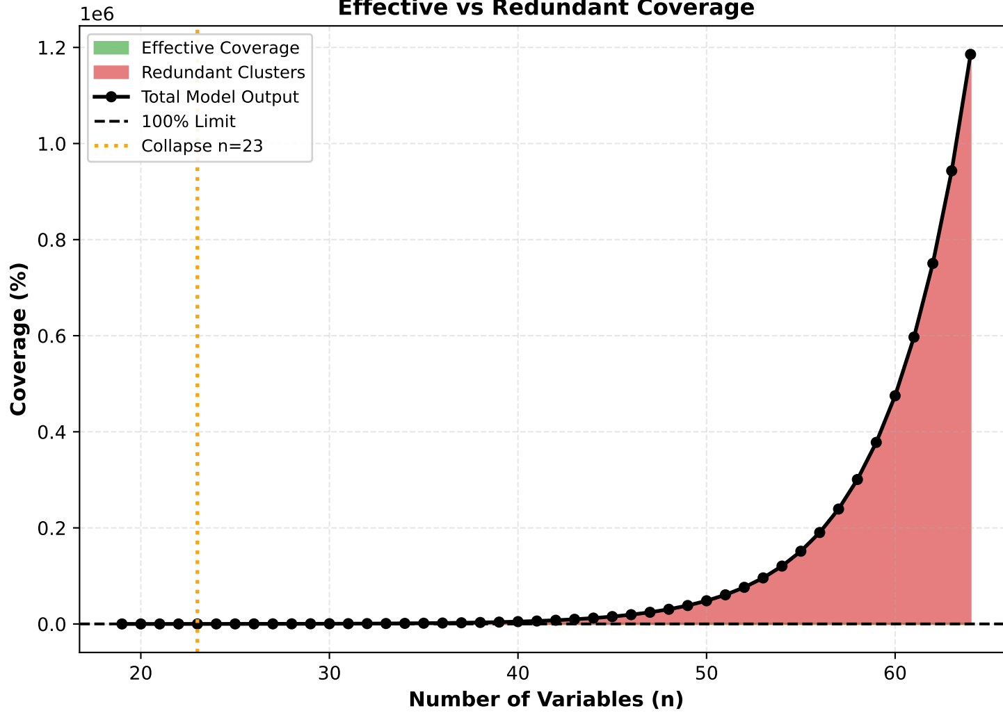
Cluster Growth
