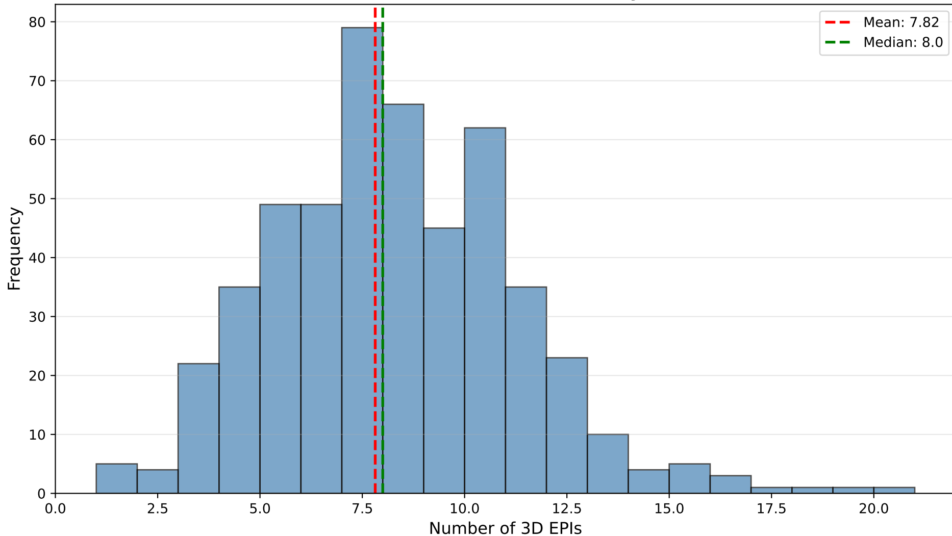
8-Variable Functions (50% density, N=500)
