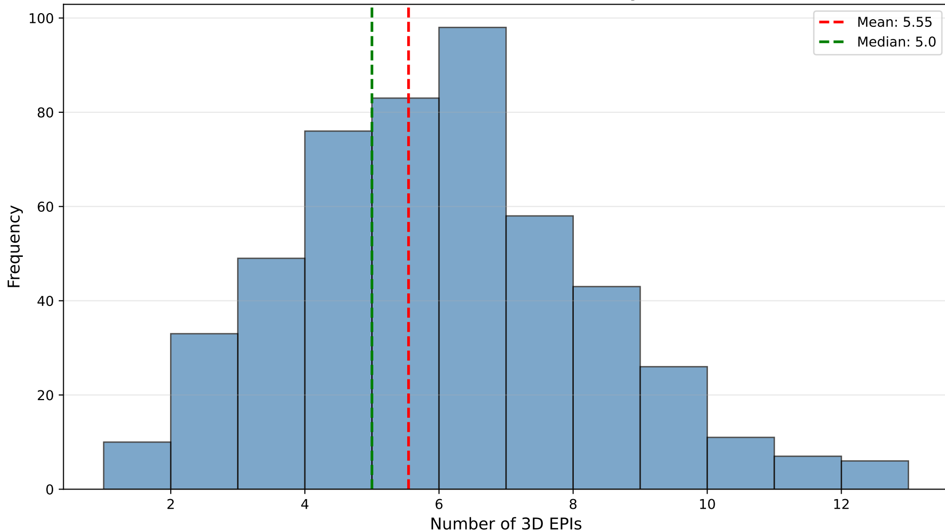
8-Variable Functions (30% density, N=500)
