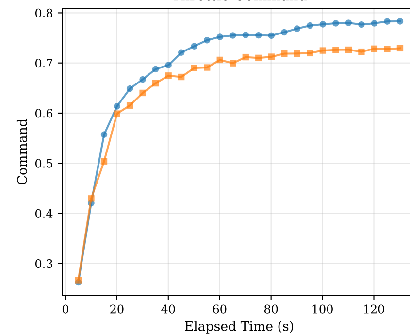
Throttle Command
