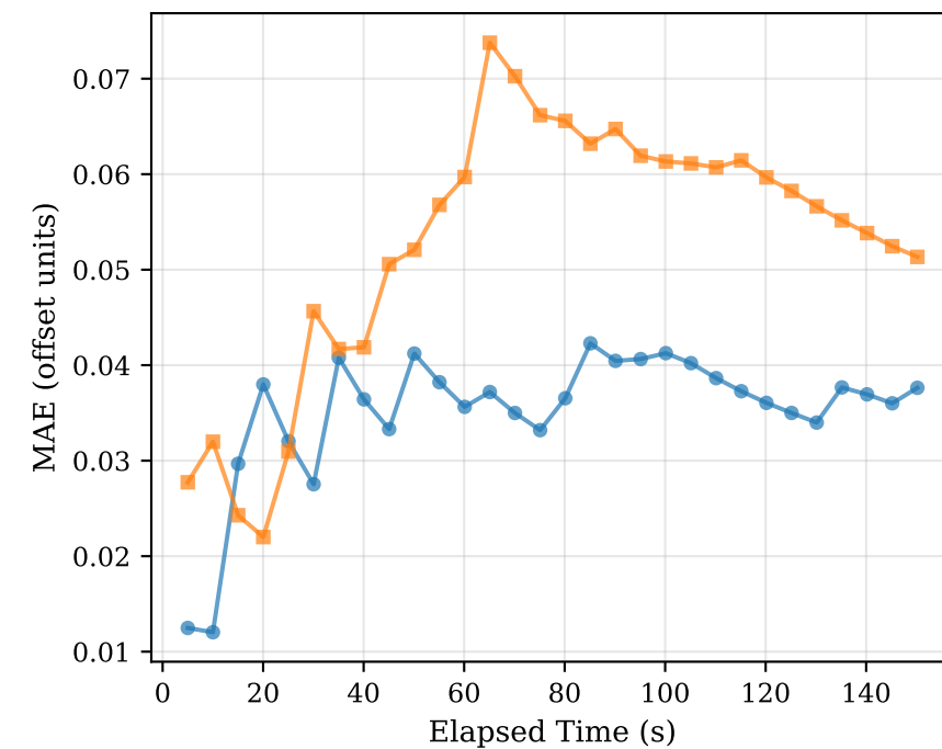
Prediction MAE
