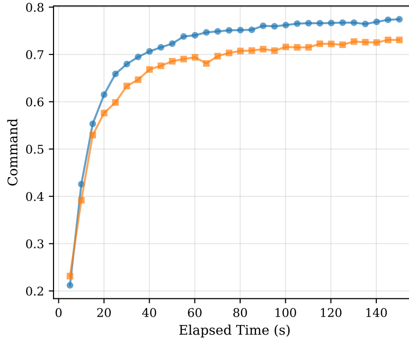
Throttle Command
