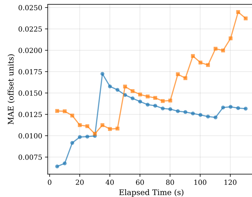
Prediction MAE
