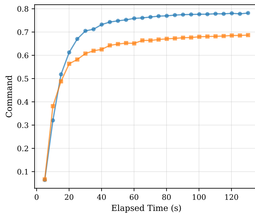
Throttle Command
