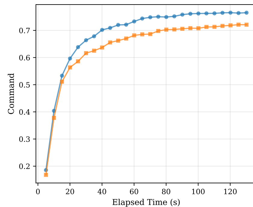
Throttle Command
