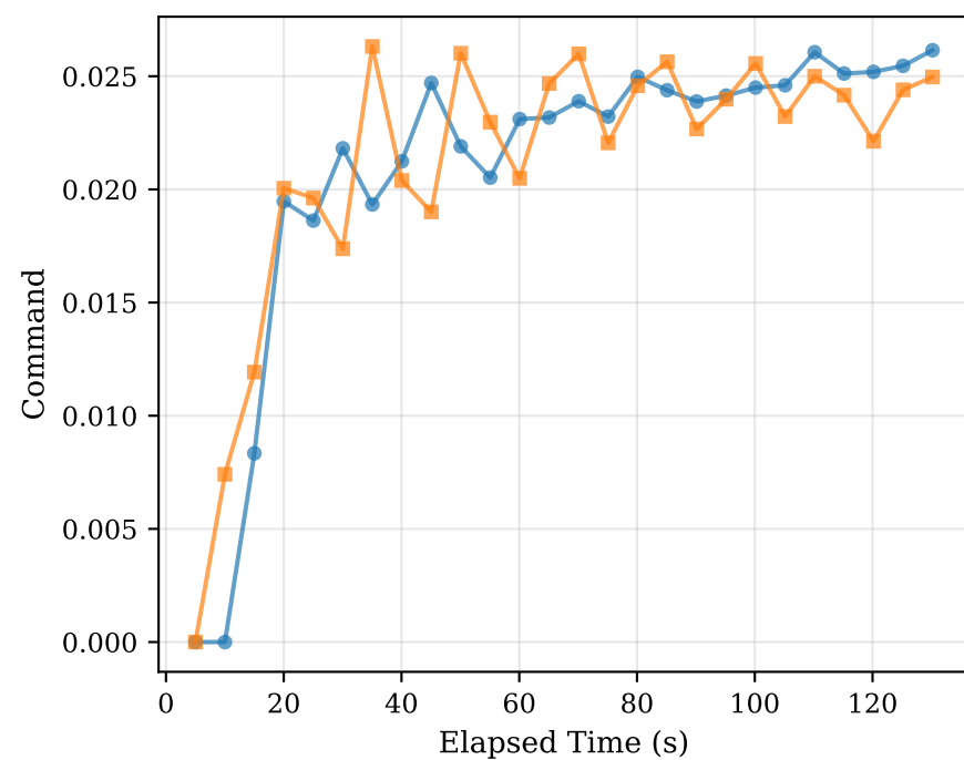
Steer Command
