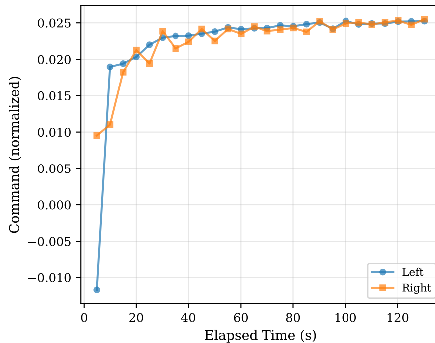
Steer Command
