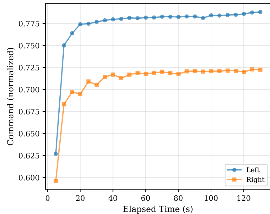
Throttle Command
