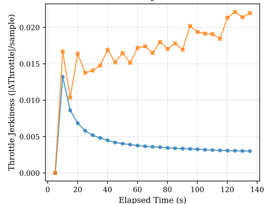
Throttle Jerkiness
