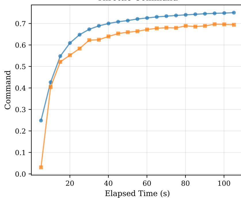
Throttle Command
