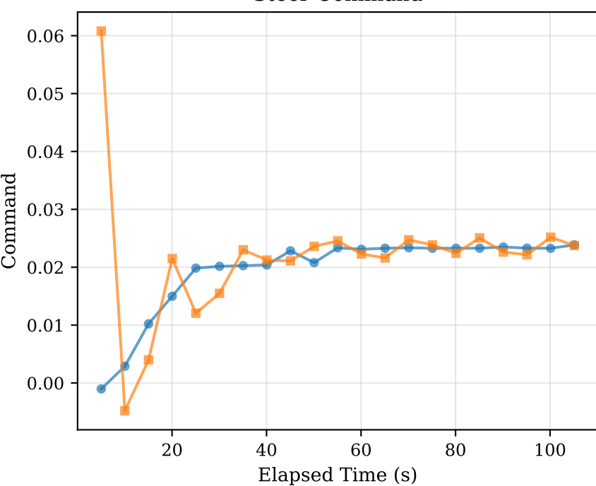
Steer Command
