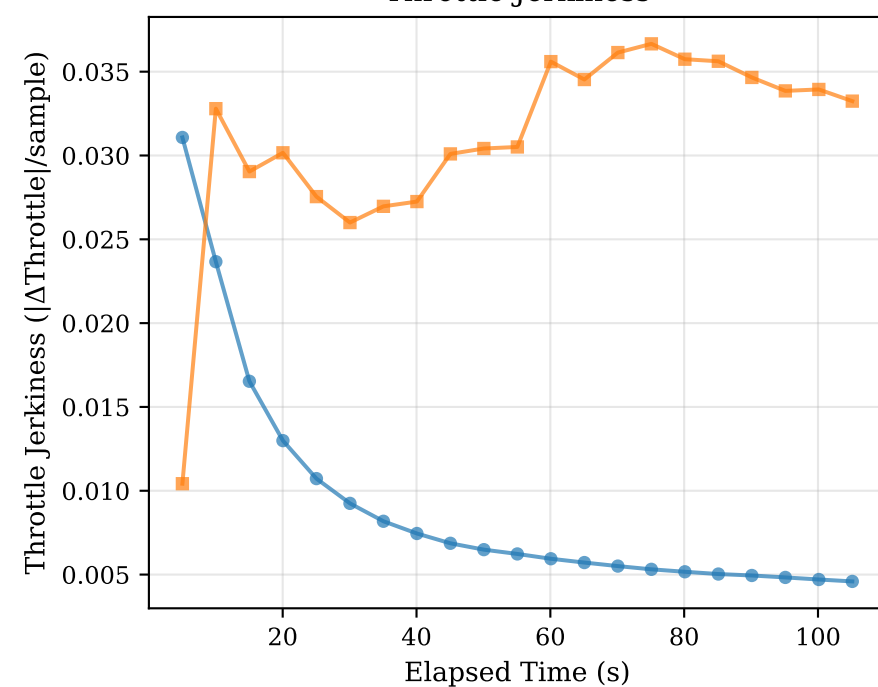
Throttle Jerkiness
