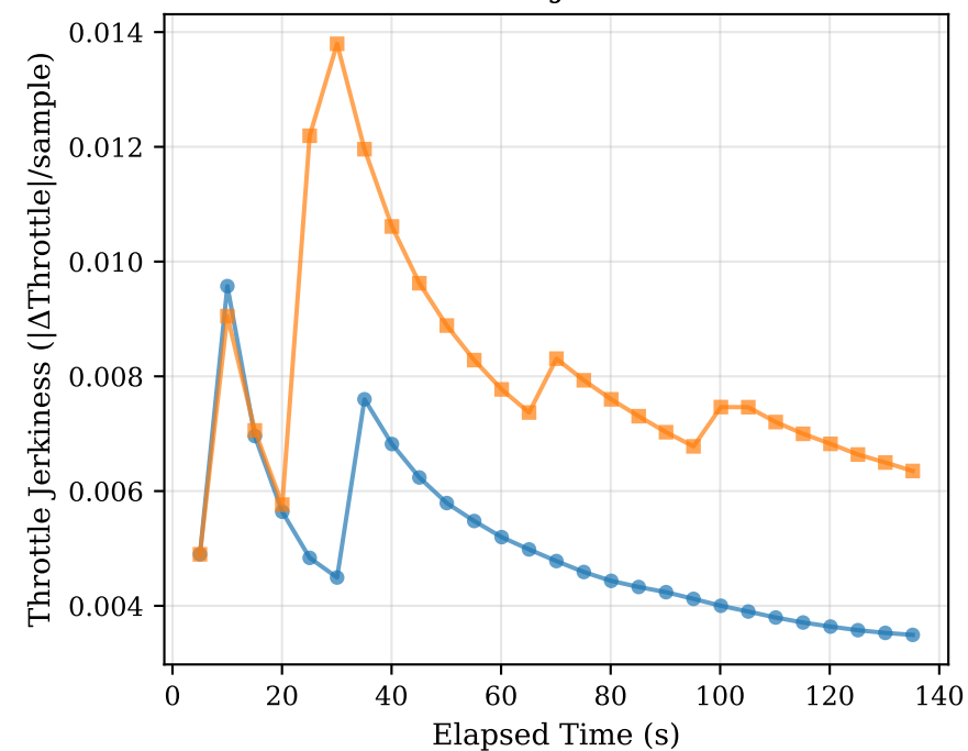
Throttle Jerkiness
