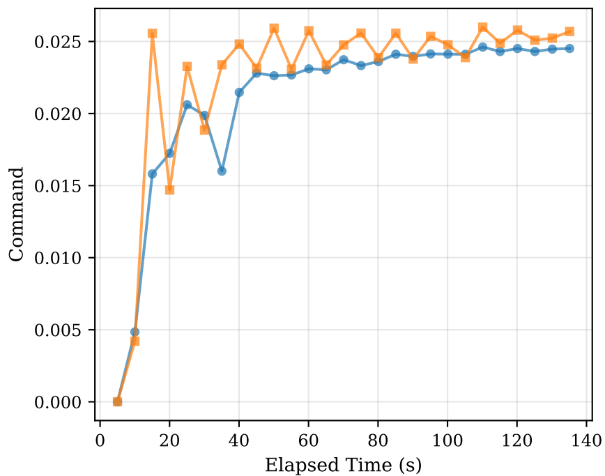
Steer Command
