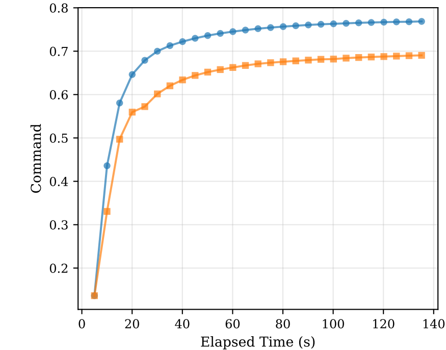
Throttle Command
